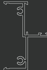
SIDELIGHT FRAME
